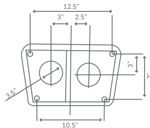
BOTTOM ANCHORING PLATE
