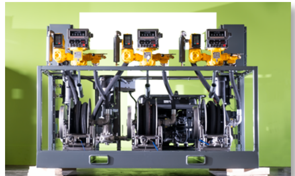
PRO-6000 BULK OIL TRANSFER SYSTEM
